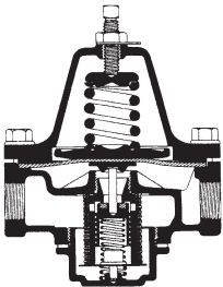
TYPE B Pressure regulator/water and air
