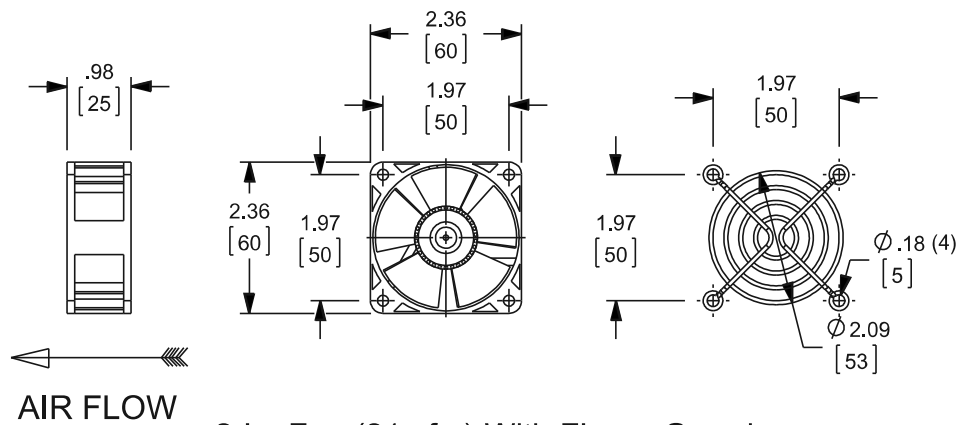
2-in. Fan (21 cfm) With Finger Guard Catalog no.: A2AXFN24
