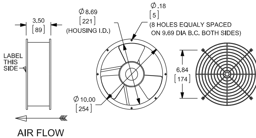
10-in. Fan (560 cfm) With Finger Guard Catalog no.'s: A10AXFN, A10AXFN2, A10AXFNPG
